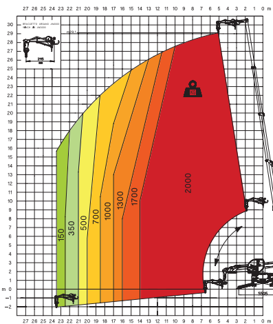
JW 2000 Jib winch 2.000
